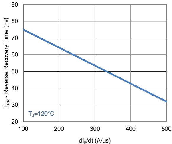
8. Reverse Recovery Time vs. di_F/dt
