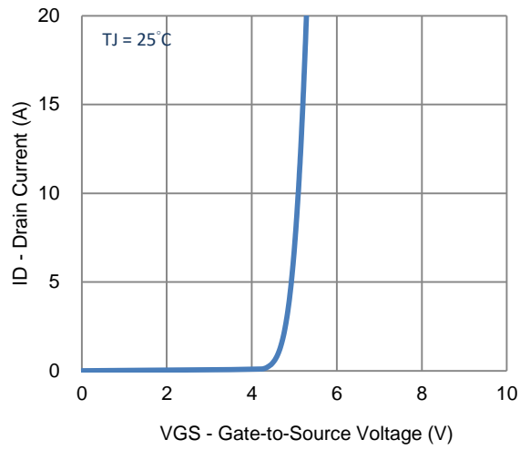
2. Transfer Characteristics
